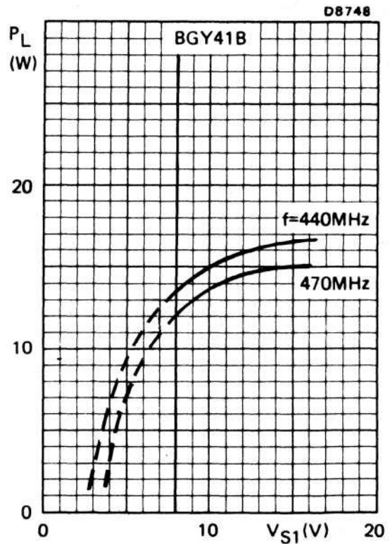
Fig.14 Typical values; V_{S2} = 12.5 V; P_D = 150 mW
