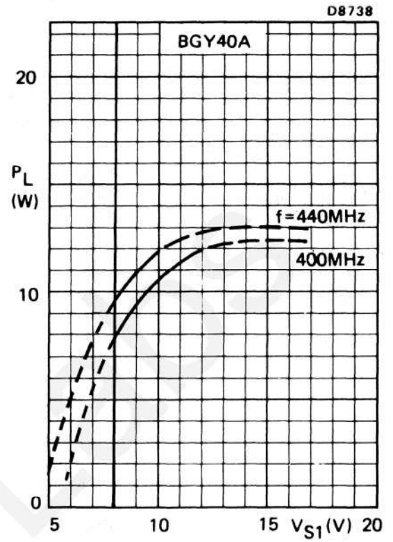
Fig.4 Typical values; V_{S2} = 12.5 V; P_D = 100 mW
