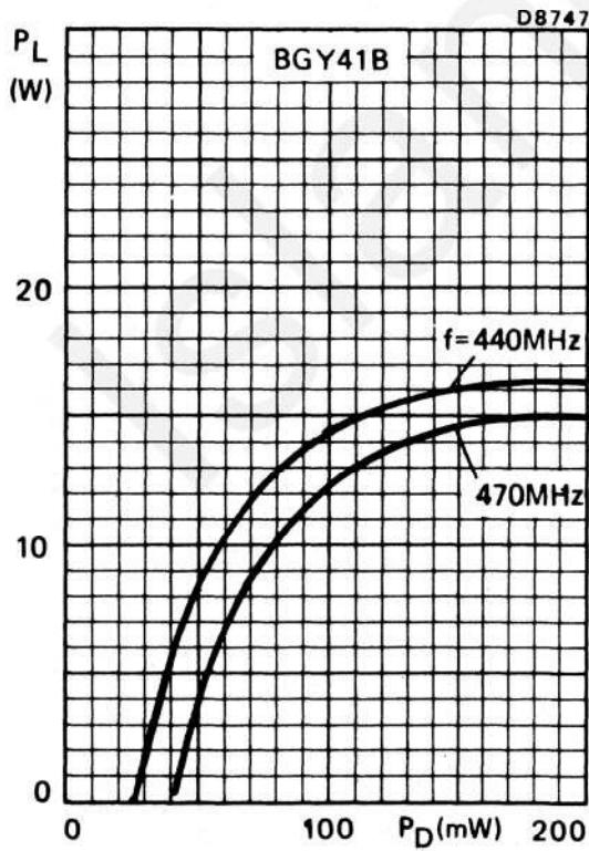
Fig.13 Typical values; V_{S1} = V_{S2} = 12.5 V
