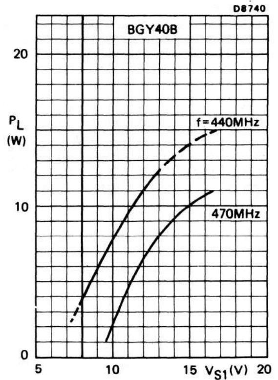
Fig.6 Typical values; V_{S2} = 12.5 V; P_D = 100 mW
