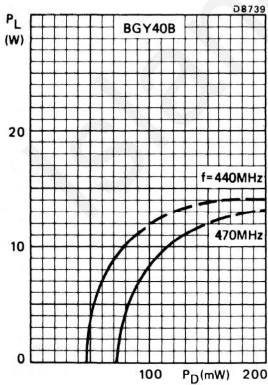
Fig.5 Typical values; V_{S1} = V_{S2} = 12.5 V
