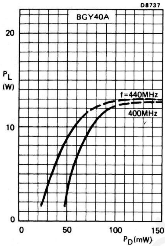
Fig.3 Typical values; V_{S1} = V_{S2} = 12.5 V
